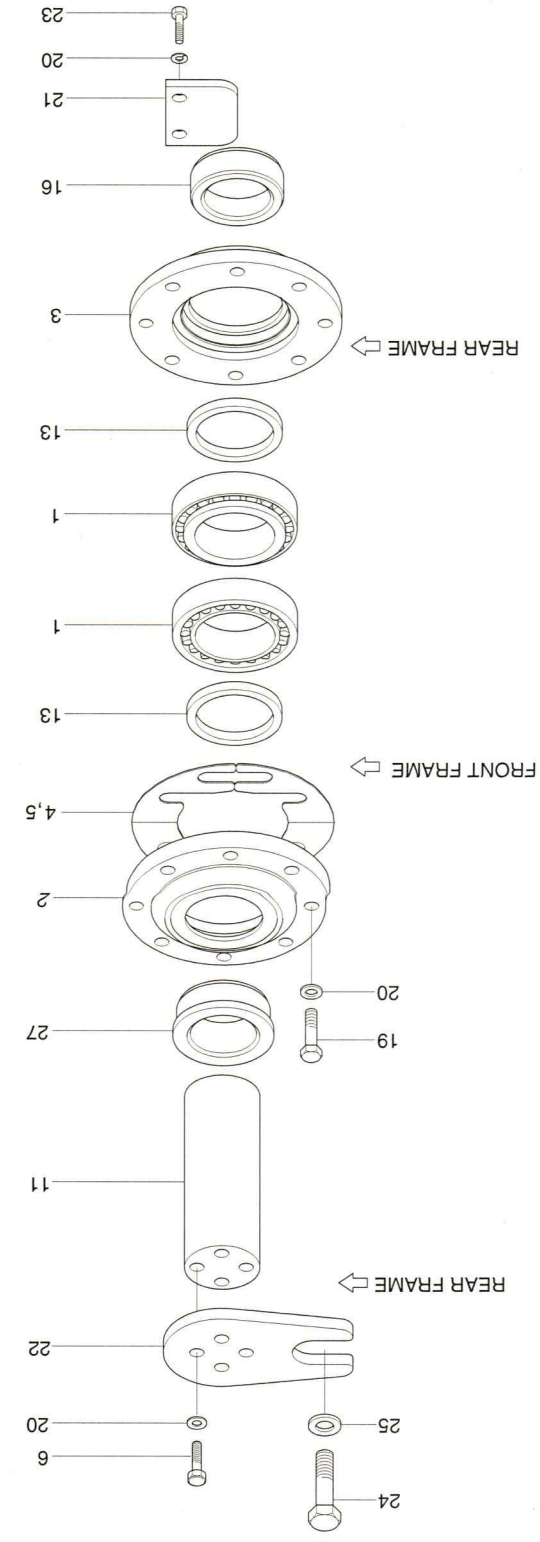
CENTER PIVOT PIN(UPPER)
